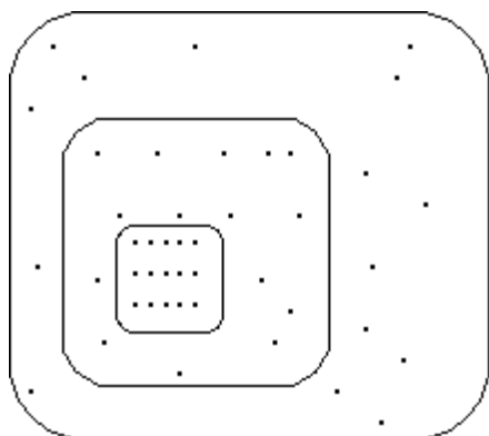
Figure 1: Bradford scatter of journal articles across three zones.
