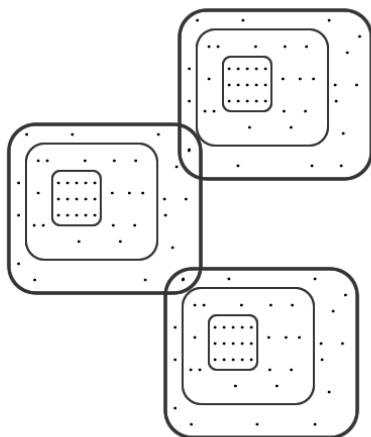
Figure 2. Bradford diagram for a multidisciplinary field.
