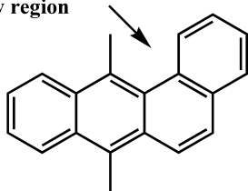
dimethylbenz[ a ]anthracene
