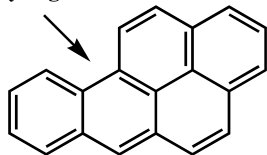
Benzo[ a ]pyrene
